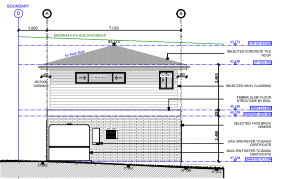
4 WEST ELEVATION 1:200
