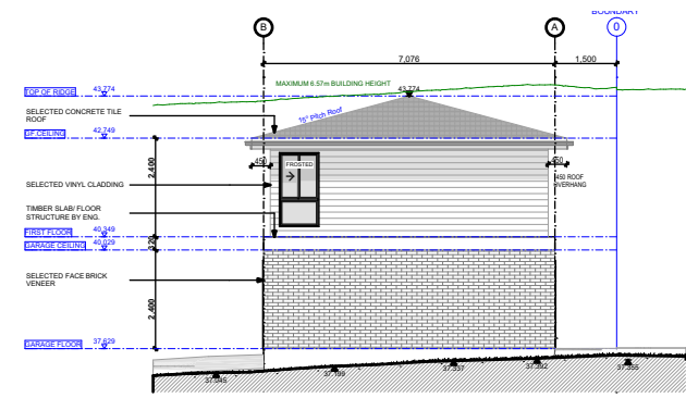
5 EAST ELEVATION 1:200
