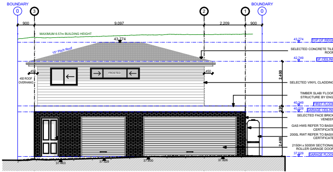
2 NORTH ELEVATION 1:200
